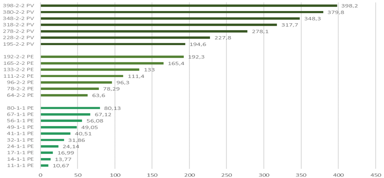
AURA HEI - Cooling capacity (kW)
